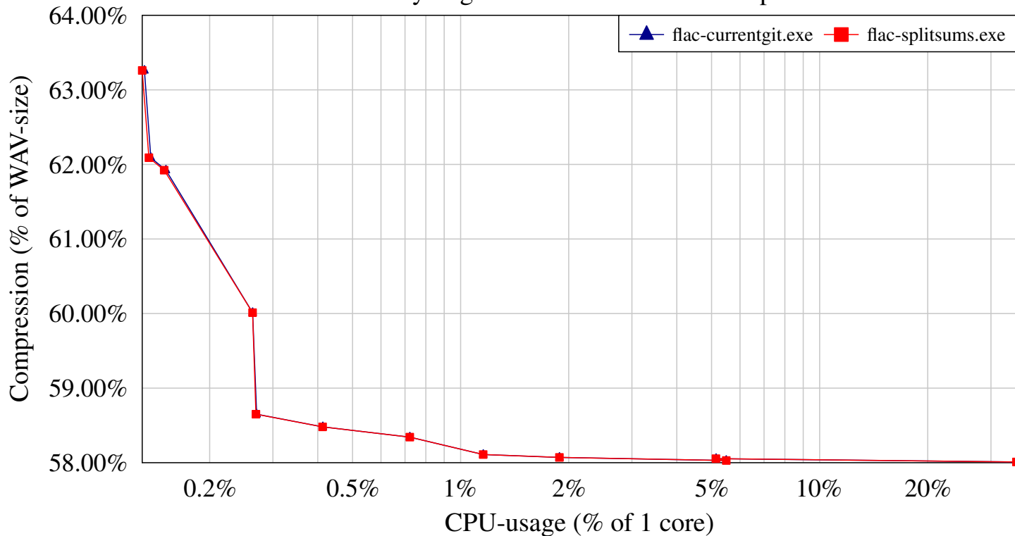
Encoding CPU-time vs compression for very large set of tracks - doublesumpatch
